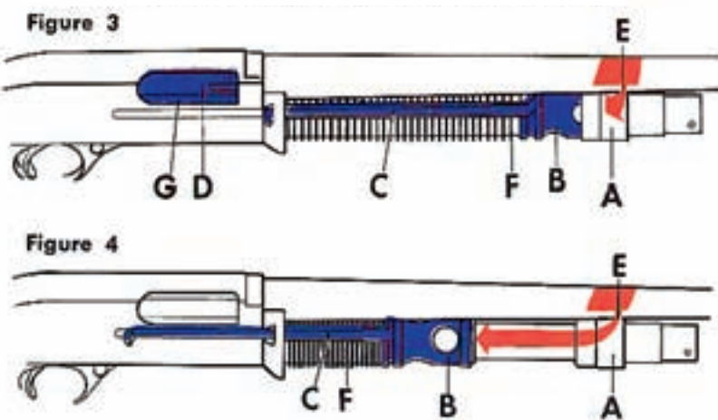
J. C. HIGGINS MODEL 60 GAS-OPERATED SHOTGUN
